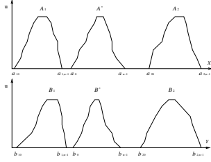
Figure 5: Interpolation with arbitrarily polygonal fuzzy membership functions
